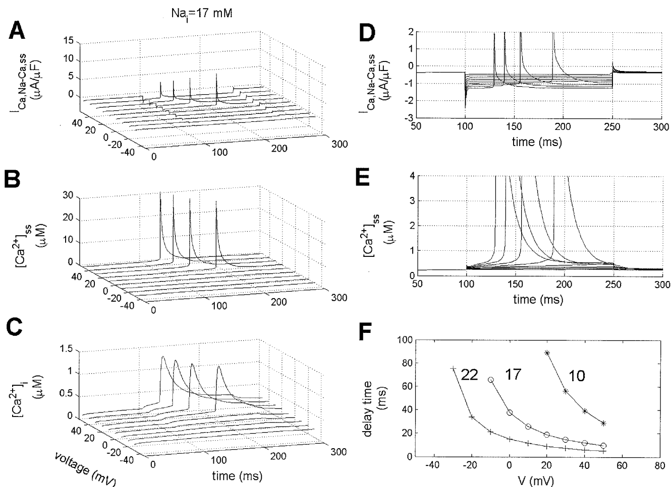
FIGURE 5 Voltage-clamp simulation with increased [Na]_i (17 mM) and without functional L-type calcium current. The voltage-clamp protocol is the same as in Fig. 4. (A) I_{Ca,Na-Ca} ; (B) calcium concentration in subpace [Ca]_{ss} ; (C) calcium concentration in the cytoplasm [Ca]_i . With increased intracellular sodium the Ca^{2+} releases are now triggered. (D and E) A closer examination of the I_{Ca,Na-Ca} and the Ca_{ss} . Note that the calcium transients (E) are triggered at different times after the beginning of the stimulus pulse (at 100 ms), depending on the amplitude of the voltage pulse. (F) The sodium- and voltage-dependence of the delay for triggering Ca^{2+} release from intracellular calcium stores with the presence of L-type Ca^{2+} channels. The delay time is defined as the duration between depolarization (leading edge of the voltage-clamp pulse) and the onset of the calcium transient. The delay is shown for three different levels of [Na]_i : (*) 10 mM, (○) 17 mM, and (+) 23 mM.
