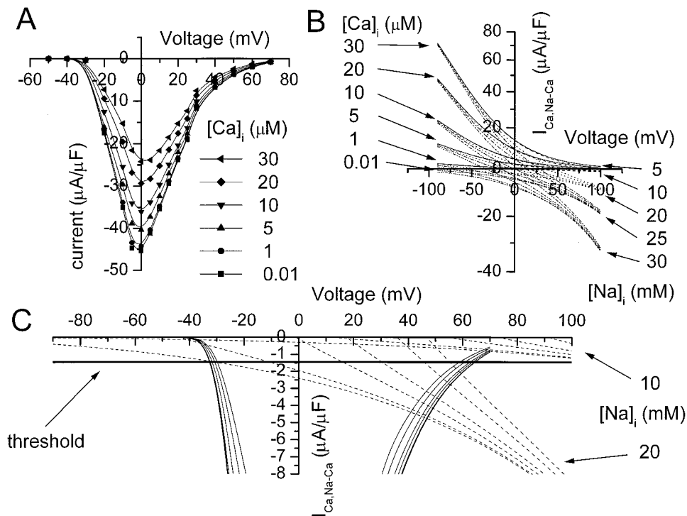
FIGURE 3 The current-voltage ( I - V ) characteristics of the L-type Ca 2+ current and the reverse mode of the Na + -Ca 2+ exchanger in varying intracellular concentrations of calcium and sodium. (A) The I - V relation of the L-type Ca 2+ current in different intracellular Ca 2+ concentration (from 0.01 to 30 μM, as indicated by different symbols). (B) The I - V relation of the Ca 2+ flux via Na + -Ca 2+ exchanger ( I_{Ca,Na-Ca} ) and its dependence on [Ca] i and [Na] i . Because the ratio of the exchange for the Na + -Ca 2+ exchanger is 3 Na + :1 Ca 2+ , the current becomes I_{Ca,Na-Ca} = -2I_{Na-Ca} . First, the [Na] i has a large influence on the I_{Ca,Na-Ca} at very positive membrane potentials (from ~+50 to 100 mV), where [Ca] i has little effect, and thus the curves tend to converge. Second, [Ca] i mainly influences I_{Ca,Na-Ca} at fairly negative potentials (from -50 to -90 mV), where [Na] i has little influence, and the curves again tend to converge. [Ca 2+ ] and [Na + ] concentrations used are shown beside the corresponding curves. (C) Combination of the two I - V relation curves ( I_{Ca,L} and I_{Ca,Na-Ca} ) and a comparison with the I_{ss,th} (the threshold of Ca 2+ influx via the sarcolemma to the restricted subspace for triggering the Ca 2+ release via RyR receptor from SR; continuous horizontal line). All values of the I - V curves below the threshold will cause CICR. Note that I_{Ca,Na-Ca} is always smaller than the threshold ( I_{ss,th} ) when [Na] i is 10 mM, but I_{Ca,Na-Ca} is significantly larger with increasing [Na] i from 10 to 20 mM.
